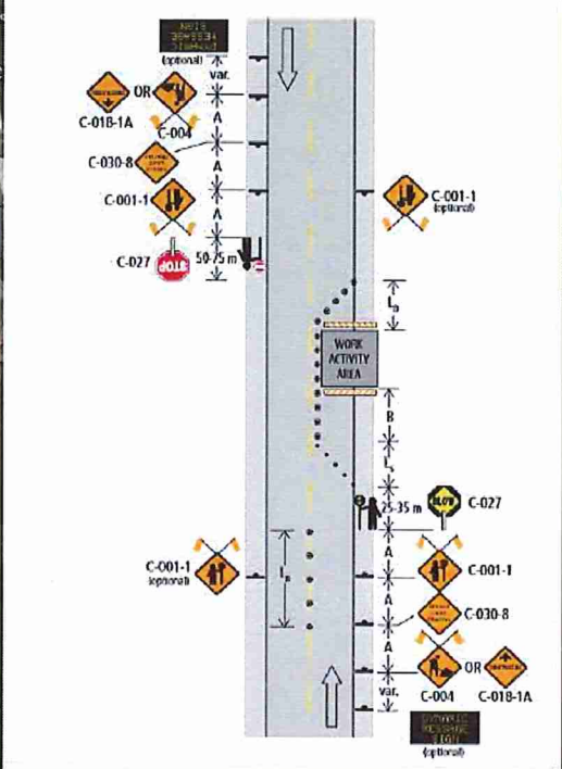
Figure 7.0: Lane Closure with TCPs – Single Lane Alternating – Short and Long Duration
